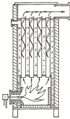
#1 VERTICAL BOILER
