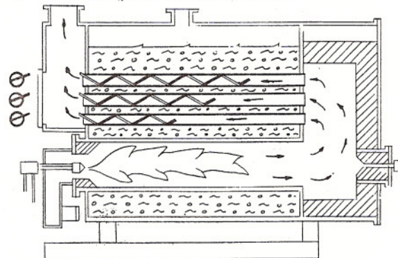
#5 2-PASS DRY BACK SCOTCH MARINE
