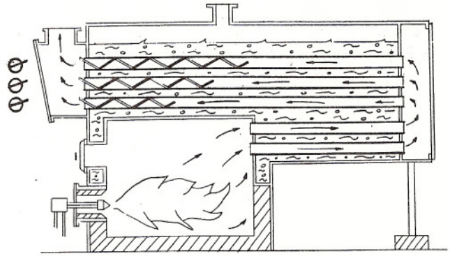
#6 FIREBOX ECONOMY BOILER
