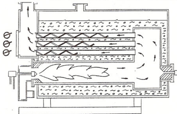
#4 2-PASS WET BACK SCOTCH MARINE
