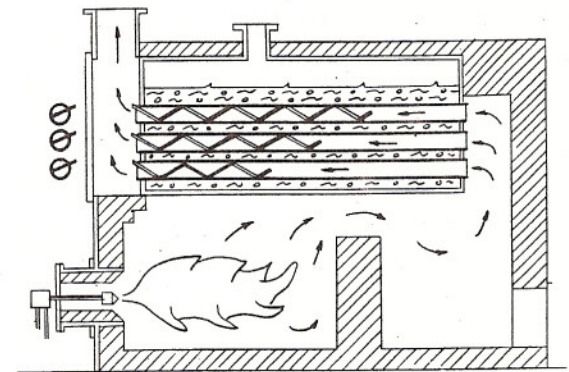
#10 H.R.T. BRICKSET BOILER
