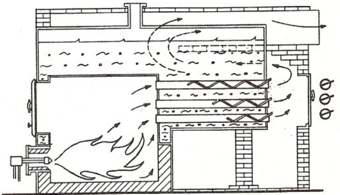
#9 FIREBOX BRICKSET BOILER
