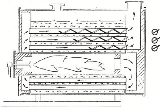
#3 3-PASS DRY BACK SCOTCH MARINE
