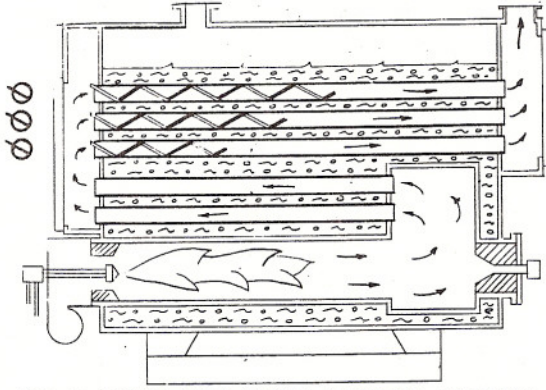
#2 3-PASS WET BACK SCOTCH MARINE
