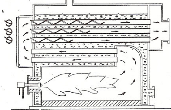
#7 FIREBOX BOILER TYPE "C"
